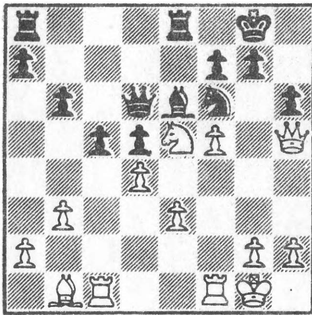
441 After 20...Nf6
